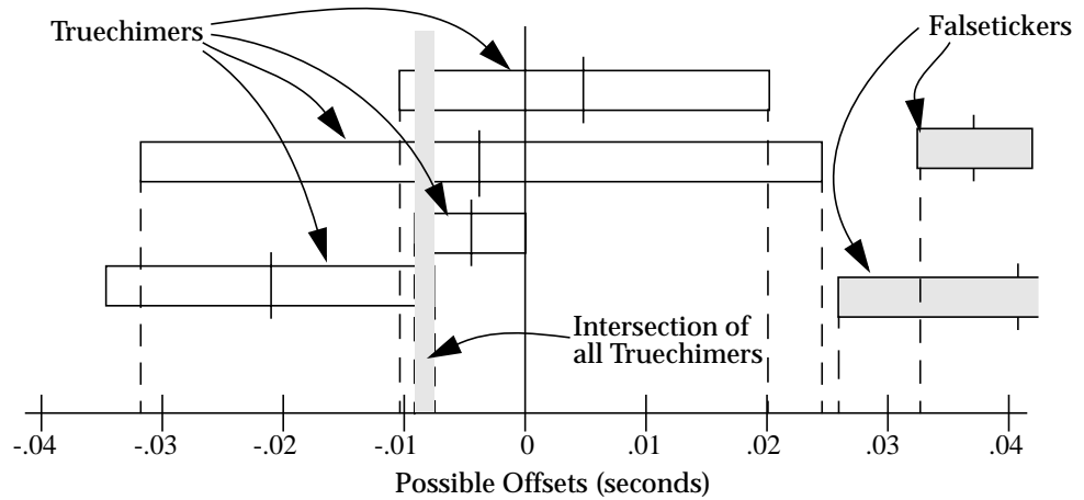
FIGURE 3 The Intersection Algorithm
