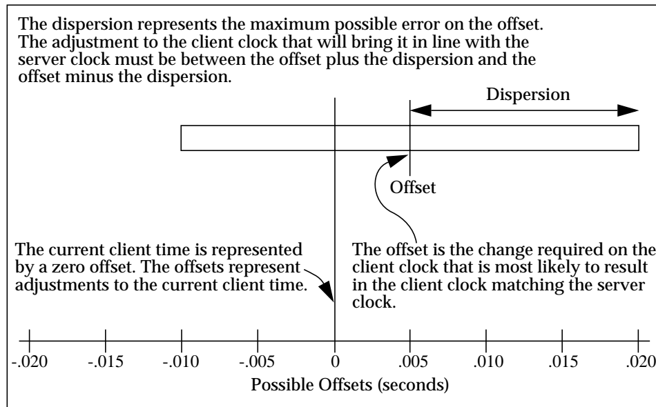
FIGURE 1 Clock Offset and Dispersion
