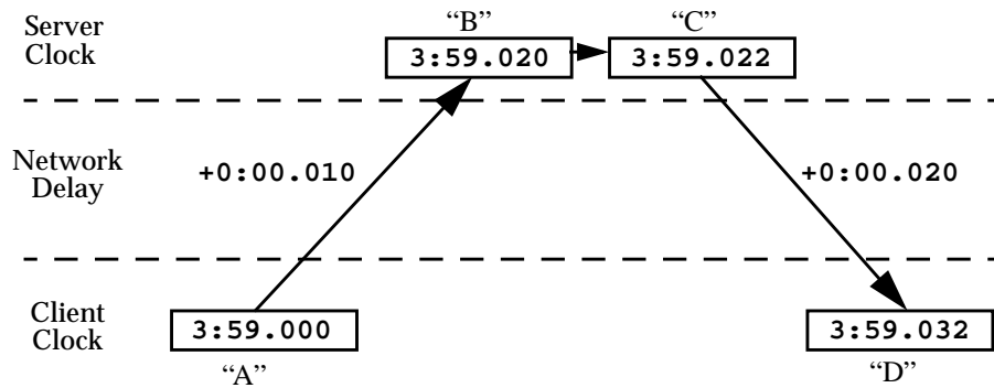
FIGURE 2 Sample Client/Server Exchange
